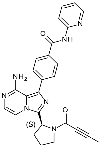
Figure 3 Chemical structure of acalabrutinib
