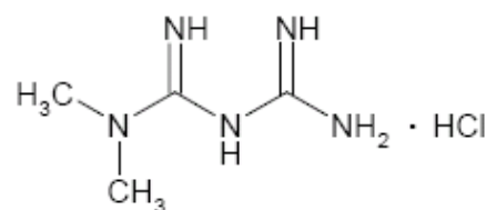
Metformin hydrochloride
