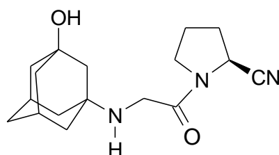
Vildagliptin
