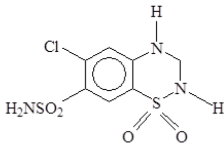
Figure 2 Chemical structure of hydrochlorothiazide
