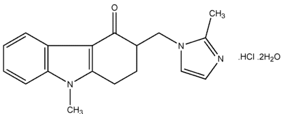
Ondansetron hydrochloride dihydrate
